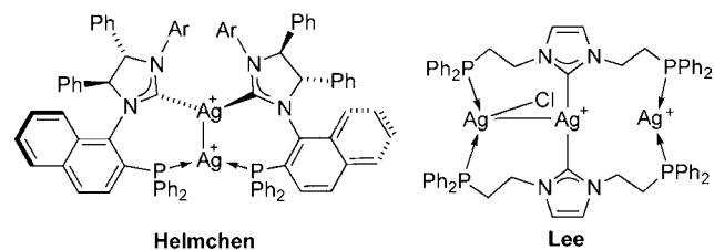
Chart 3. Previously Reported Ag(I) Complexes with P-NHC Hybrid Ligands Used for Transmetalation Reactions
