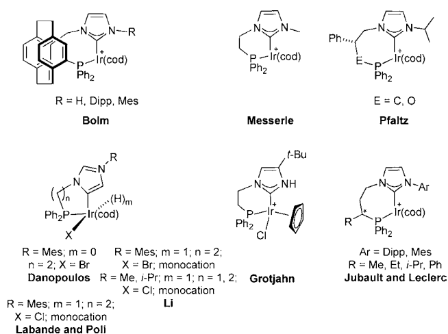
Chart 5. Relevant Ir Complexes with P-NHC Hybrid Ligands (See Text)
