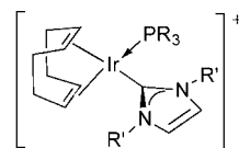
Chart 4. General Formula of Ir Complexes Containing Monodentate Phosphine and NHC Ligands
