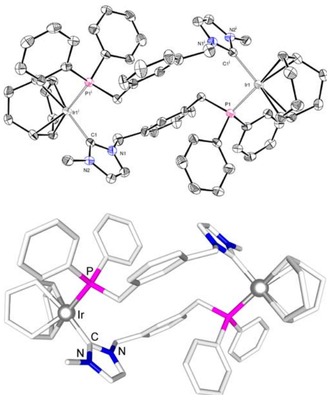
Figure 2. Top: ORTEP of the molecular structure of the dicationic complex [\text{Ir}(\text{cod})(\mu\text{-P-NHC},\kappa\text{P},\kappa\text{C}_{\text{NHC}})]_2 in 4\cdot 2\text{THF} with 30% probability thermal ellipsoids. The 2 molecules of THF, the anions, and the hydrogen atoms have been omitted for clarity. Selected bond lengths [Å] and angles [deg]: Ir1i–C1 2.043(7), Ir1i–P1i 2.316(2); C1–Ir1i–P1i 91.5(2), N1–C1–N2 104.0(6). Bottom: Perspective view of the molecular structure of the dicationic complex in 4 (Diamond software).
