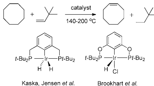
Scheme 10. Transfer Dehydrogenation of coa in the Presence of the
