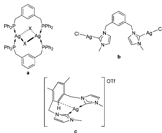
Chart 6. Ag(I) Complexes with Phosphorus or NHC Ligands Related to the Hybrid Ligand Present in 3
