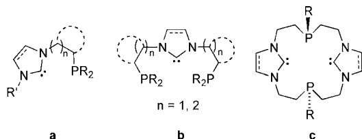
Chart 2. Examples of Hybrid Phosphine-NHC Ligands
