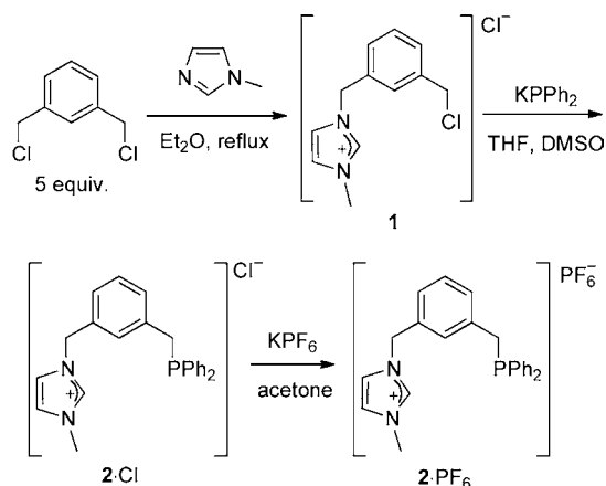
Scheme 1. Synthesis of the Phosphine-Imidazolium Precursor
