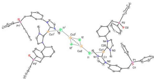
Figure 5. ORTEP of the Cu(I) complex 13 with 30% probability thermal ellipsoids. Hydrogen omitted for clarity. Selected bond lengths [Å] and angles [deg]: Cu1–C1 1.912(8), Cu1–C26 1.930(9), Cu1–I1 3.119(1), Cu2–I1 2.522(2), Cu2–I2, 2.576(2); C1–Cu1–C26 162.6(4), C1–Cu–I1 97.7(3), Cu1–I1–Cu2 121.99(5), I2–Cu2–I2' 108.37(6).
