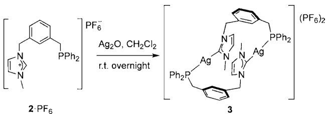
Scheme 2. Synthesis of the Ag(I) Complex [\text{Ag}(\mu\text{-P-NHC}, \kappa\text{P}, \kappa\text{C}_{\text{NHC}})]_2(\text{PF}_6)_2 ( 3 )
