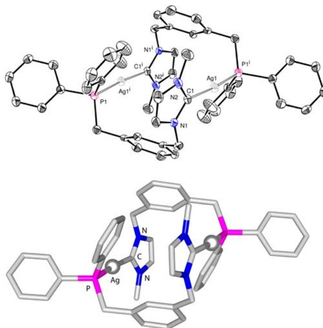
Figure 1. (top): ORTEP of the molecular structure of the dicationic complex [\text{Ag}(\mu\text{-P-NHC}, \kappa\text{P}, \kappa\text{C}_{\text{NHC}})]_2 in 3 with 30% probability thermal ellipsoids. Hydrogen atoms and anions omitted for clarity. Selected bond lengths [Å] and angles (deg): \text{Ag1-C1} 2.104(5), \text{Ag1-P1} 2.366(1); \text{C1-Ag1-P1} 172.94(2), \text{C1-N1-C3} 104.7(5). (bottom) Perspective view of the molecular structure of 3 (Diamond software).
