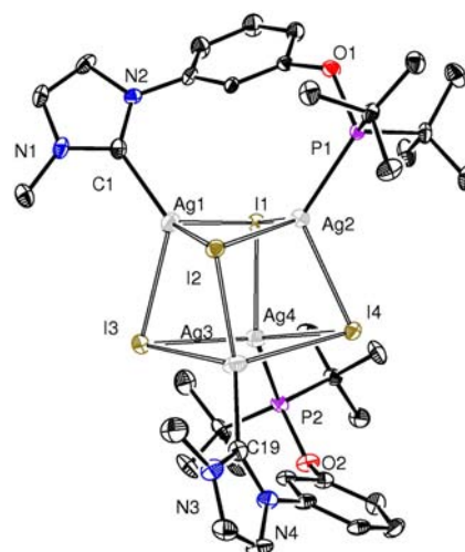
Figure 3. ORTEP of 9a in 9a- \text{CH}_2\text{Cl}_2 with 30% probability thermal ellipsoids. Hydrogen atoms omitted for clarity. Selected bond lengths [Å] and angles [deg]: Ag1–C1 2.176(8), Ag2–P1 2.451(2), Ag3–C19 2.156(9), Ag4–P2 2.460(2), Ag1–I1 2.9740(9), Ag1–I2 2.887(1), Ag1–I3 2.987(1), Ag1–Ag2 3.084(1), Ag3–Ag4 3.045(1); N1–C1–N2 103.3(7), C1–Ag1–I1 104.5(2), C1–Ag1–I2 123.4(2), C1–Ag1–I3 127.6(2), I1–Ag1–I2 113.96(3), I1–Ag1–I3 93.80(3), I2–Ag1–I3 90.29(3).
