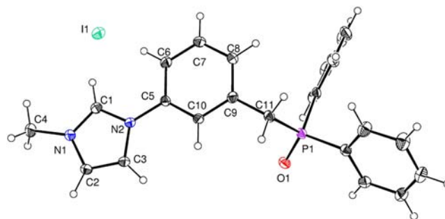
Figure 4. ORTEP of 11 with 30% probability thermal ellipsoids. Selected bond lengths [Å] and angles [deg]: N1–C1 1.312(3), N2–C1 1.337(4), P1–O1 1.483(2); N1–C1–N2 109.2(3), C11–P1–O1 114.1(1).
