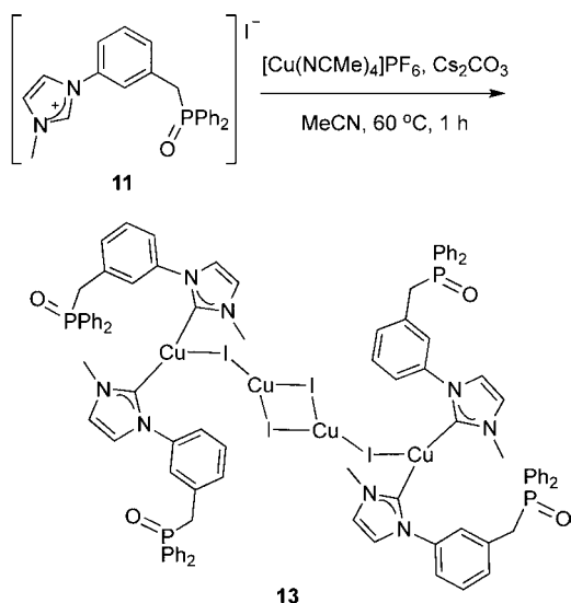
Scheme 9. Synthesis of the Tetranuclear Cu(I) Complex [\text{Cu}(\text{OP-NHC}, \kappa\text{C}_{\text{NHC}})_2(\mu\text{-I})\{\text{Cu}(\mu\text{-I})\}]_2 ( 13 )
