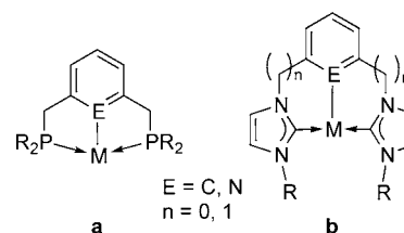
Chart 1. Pincer-Type Complexes with Phosphorus (a) or NHC Donor Groups (b)
